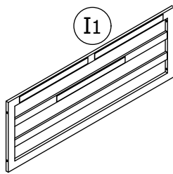
Side Guard Rail T981770 X 1
